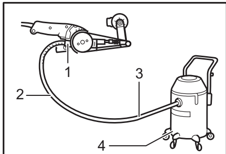
► 1. Nozzle cap 2. Hose 19 3. Hose of vacuum cleaner 4. Vacuum cleaner
